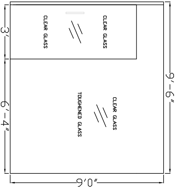
MANAGER'S CABIN :FRONT TOUGHENED GLASS PARTITION
