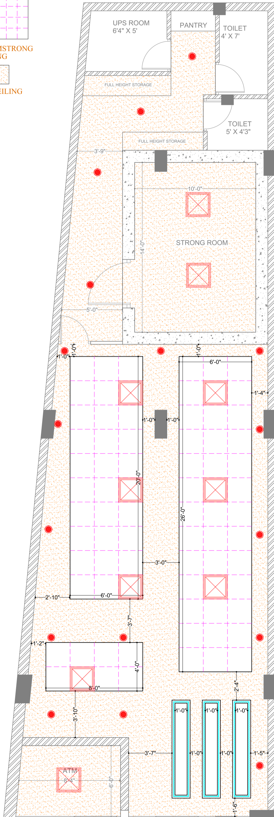
FINAL PLAN 18.10.24 FALSE CEILING PLAN
