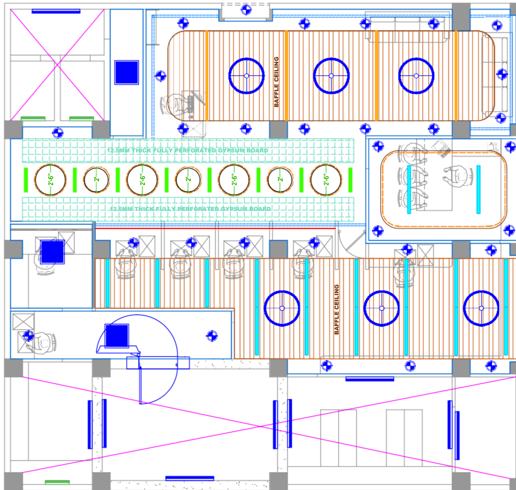
FALSE CEILING AND LIGHTING LAYOUT PLAN FOR DEULALAND MODEL BRANCH
